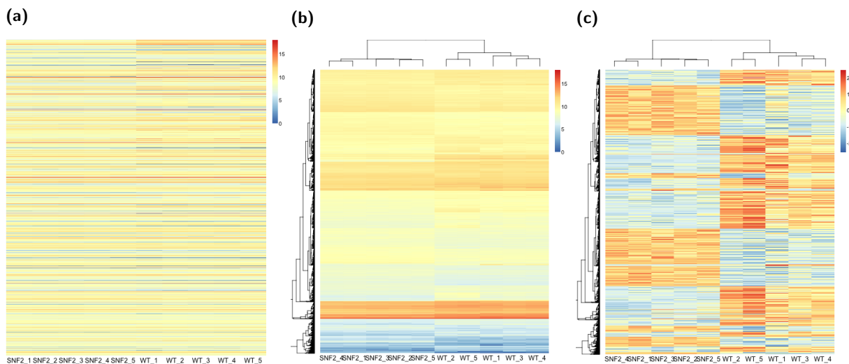
Figure 26: Heatmaps of rlog -transformed read counts for genes with adjusted p -values < 0.05 in the DGE analysis. a) Genes sorted according to the adjusted p -values of the DGE analysis. b) Genes sorted according to hierarchical clustering. c) Same as for (b), but the read count values are scaled per row so that the colors actually represent z -scores rather than the underlying read counts.
