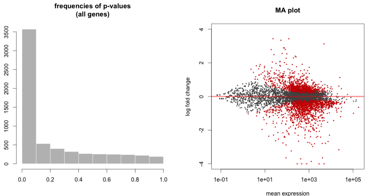
Figure 25: Left: Histogram of p -values for all genes tested for no differential expression between the two conditions, SNF2 and WT. Right: The MA plot shows the relationship between the expression change (M) and average expression strength (A); genes with adjusted p -values < 0.05 are marked in red.
