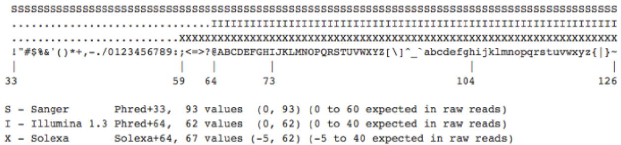
Figure 7: The ASCII interpretation and ranges of the different Phred score notations used by Illumina and the original Sanger interpretation (Table 3). Although the Sanger format allows a theoretical score of 93, raw sequencing reads typically do not exceed a Phred score of 60. In fact, most Illumina-based sequencing will result in maximum scores of 41 to 45.
