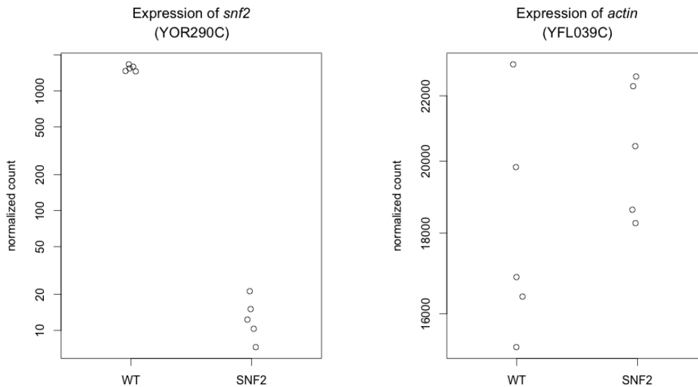
Figure 27: Read counts for snf2 and actin in the replicates of both conditions.
