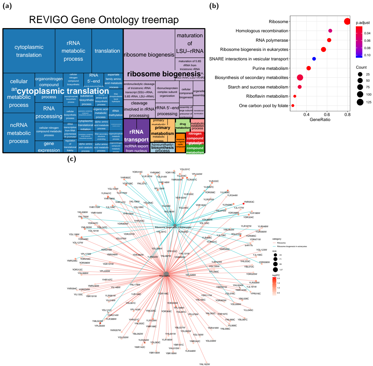
Figure 30: Example plots that may be produced following ORA with goseq and REVIGO (a) or gene set enrichment analysis using the KEGG pathways and visualizations provided by clusterProfiler (b, c). (a) Treemap generated by REVIGO to group GO terms that were determined to be enriched in our set of yeast DEG by goseq . The size of the squares corresponds to inverse of the \log(p\text{-value}) of the enrichment, the colors indicate semantically similar terms. (b) Dot plot generated with the clusterProfiler package following GSEA for KEGG pathways. Shown here are the most significantly enriched pathways. (c) Gene concept network generated with the cnetplot function of the clusterProfiler package on the same results. This plot is useful to visually assess the overlap of genes between different gene sets: the edges correspond to the membership of a given gene within a gene set (central node). See https://github.com/friedue/course_RNA-seq2019/tree/master/Day04 for the code.
