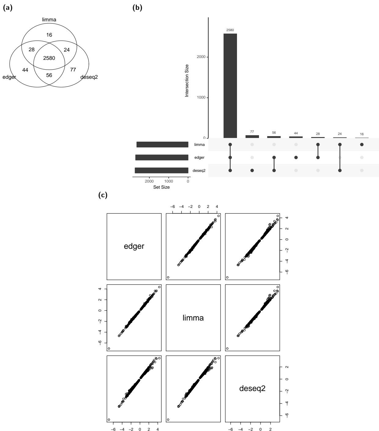
Figure 29: Some basic plots to judge the agreement of the three different DGE tools that we used. (a) Venn diagram of gene names. (b) Upset plot of gene names that displays the total size of every set in the bottom left corner, followed by the type of intersection (dots connected by lines) and the size of the intersection using vertical bars. (c) Pairwise plots of estimated/moderated log-fold-changes as determined by either one of the tools. Shown here are the genes that were identified as DE in all three tools (2,580 genes). The code used to generate those images is shown at the beginning of section 6.4.
