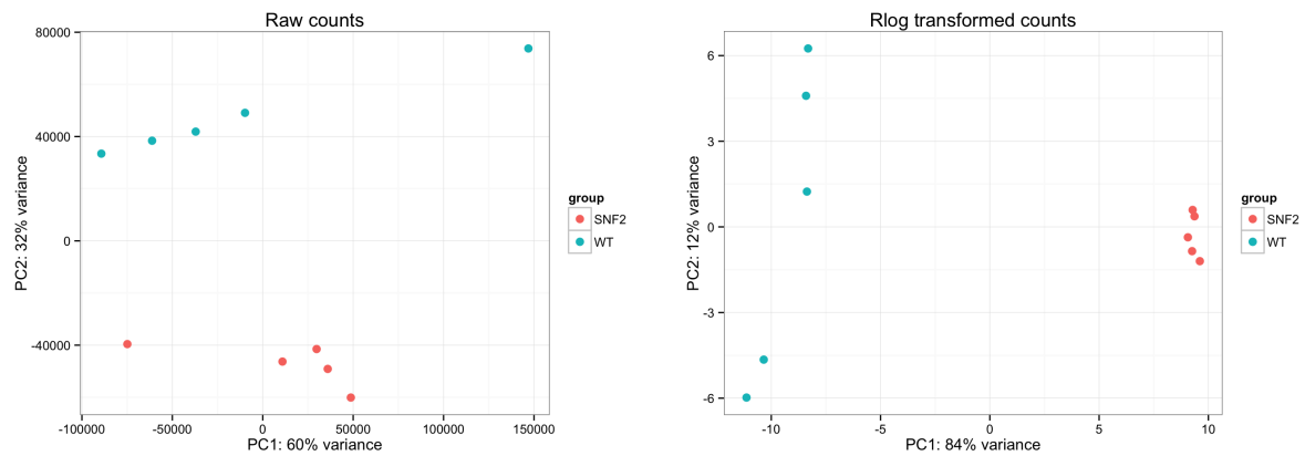
Figure 23: PCA on raw counts and rlog -transformed read counts with the DESeq2 convenience function plotPCA() . As indicated by the labels of the axes, the different sample types explain a greater fraction of the variance for rlog -transformed values than for the raw counts.
