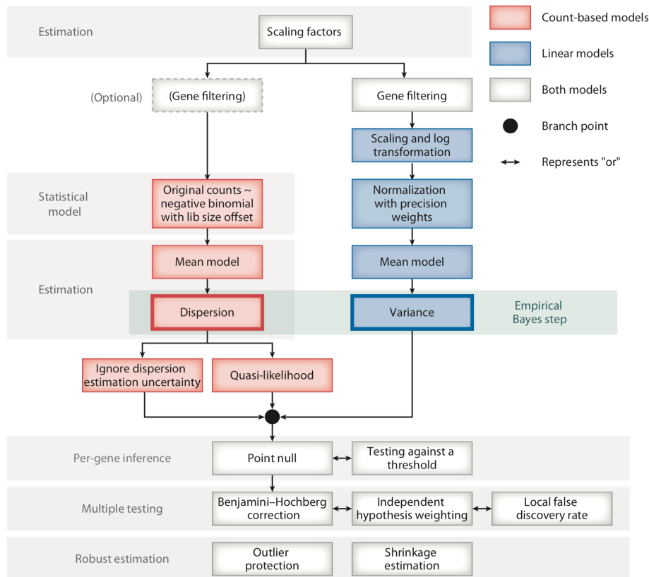
Figure 28: Schematic overview of DE analysis for RNA-seq data. Red boxes correspond to pipelines for count-based (generalized linear) models (e.g., edgeR , DESeq2 ), while blue boxes correspond to a linear-model-based pipeline as implemented by limma-voom . Figure from Van den Berge et al. (2019).
